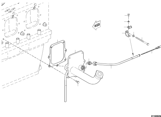
OIL DIPSTICK W/OIL FILLER NECK XS527010.00008
